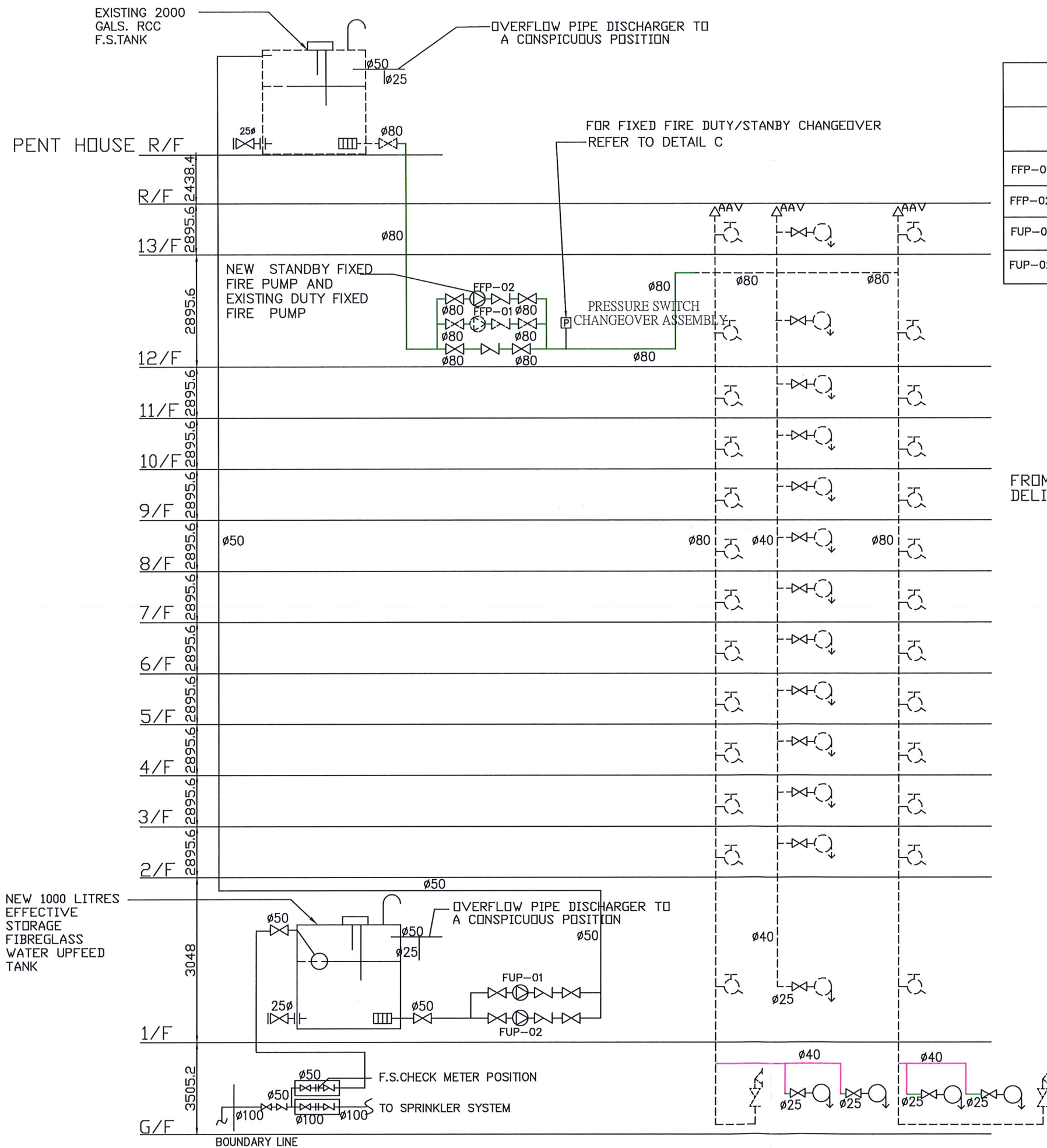
SCHEMATIC PIPING DIAGRAM FOR FH/HR SYSTEM
