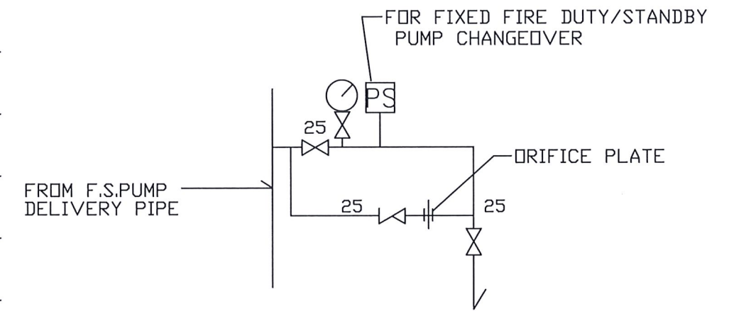
DETAIL C FOR PRESSURE SWITCH CHANGEDOVER ASSEMBLY
